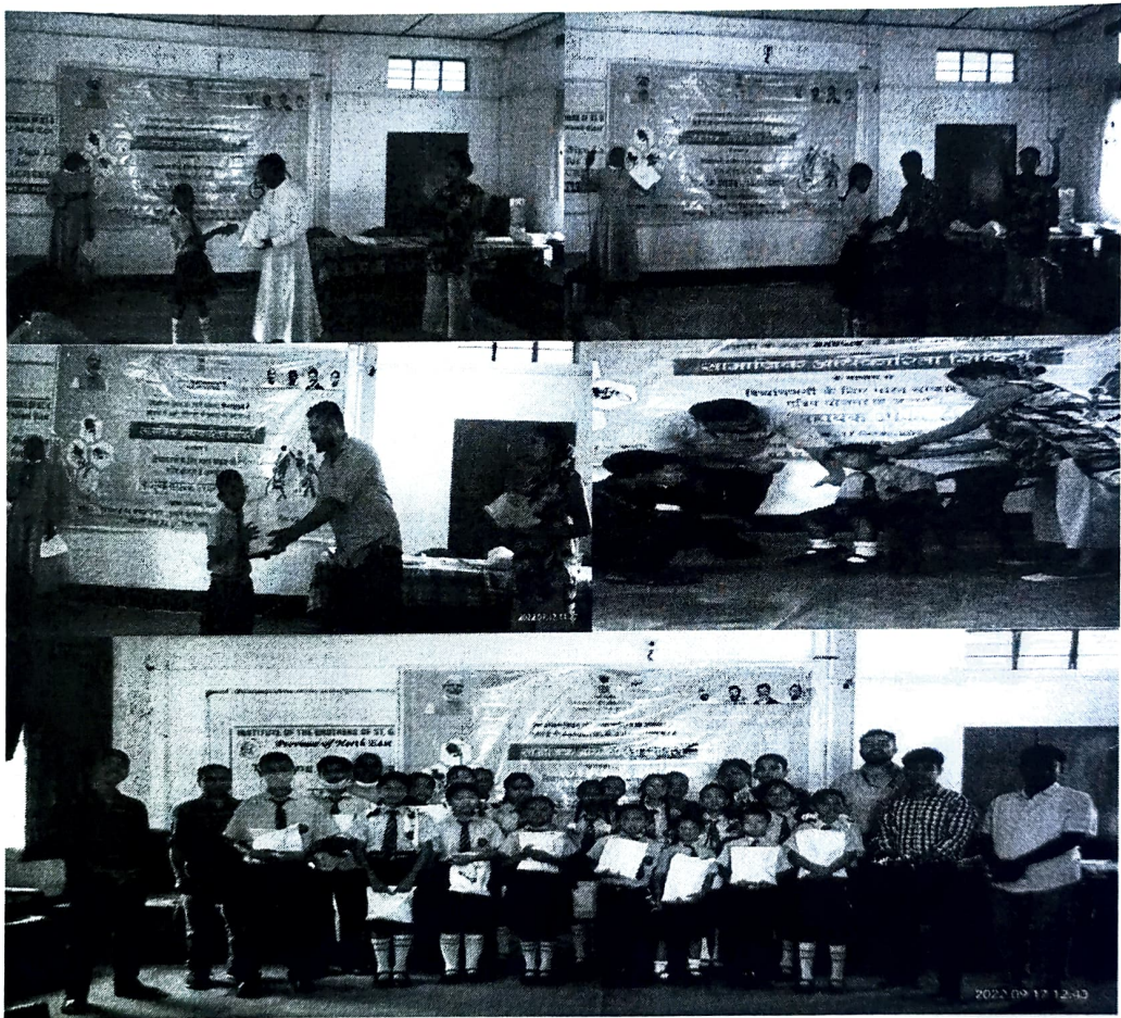
Token Distribution:
